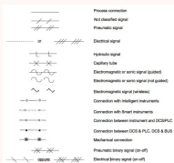
Instrumentation Symbol...
